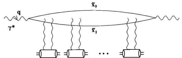
FIG. 1. Forward amplitude of DIS on a nucleus in the quasi-classical (Glauber) approximation.
