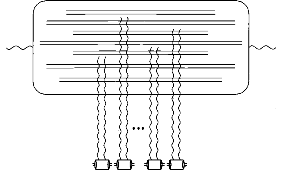
FIG. 2. DIS on a nucleus including the QCD evolution in the quark-antiquark pair in the form of dipole wave function. Each double line represents a gluon in the large- N_c limit.
